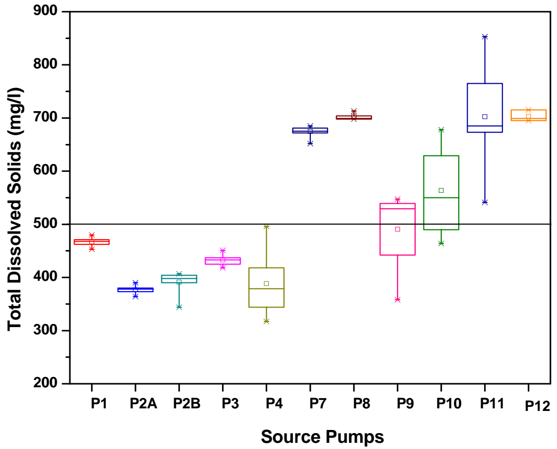
Variation of Total Dissolved Solids at Source Pumps (2011)
