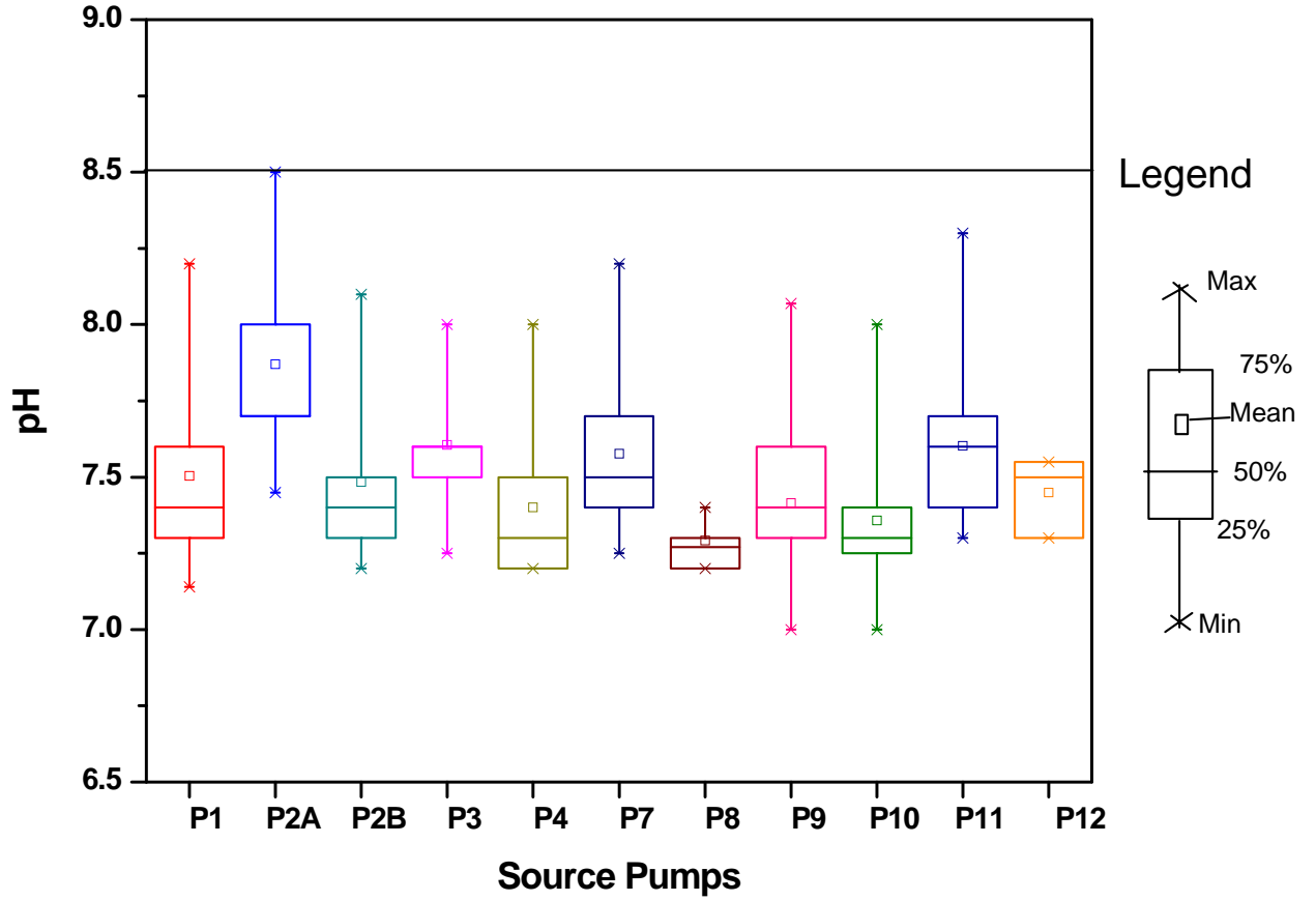
Variation of pH at Source pumps (2011)
