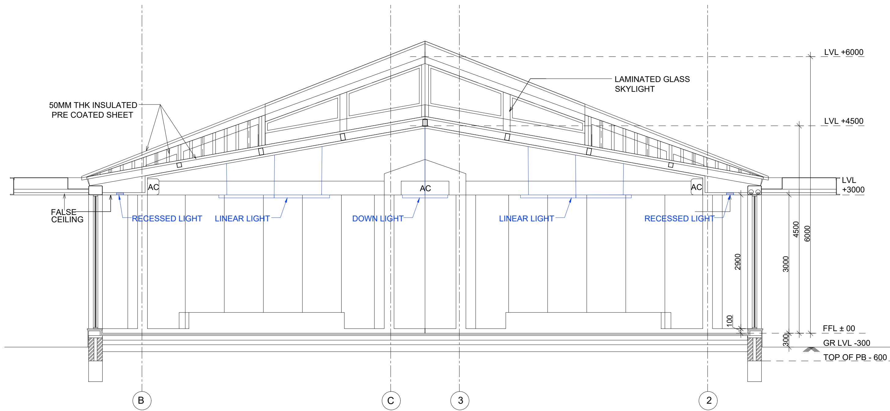
SECTION - BB
