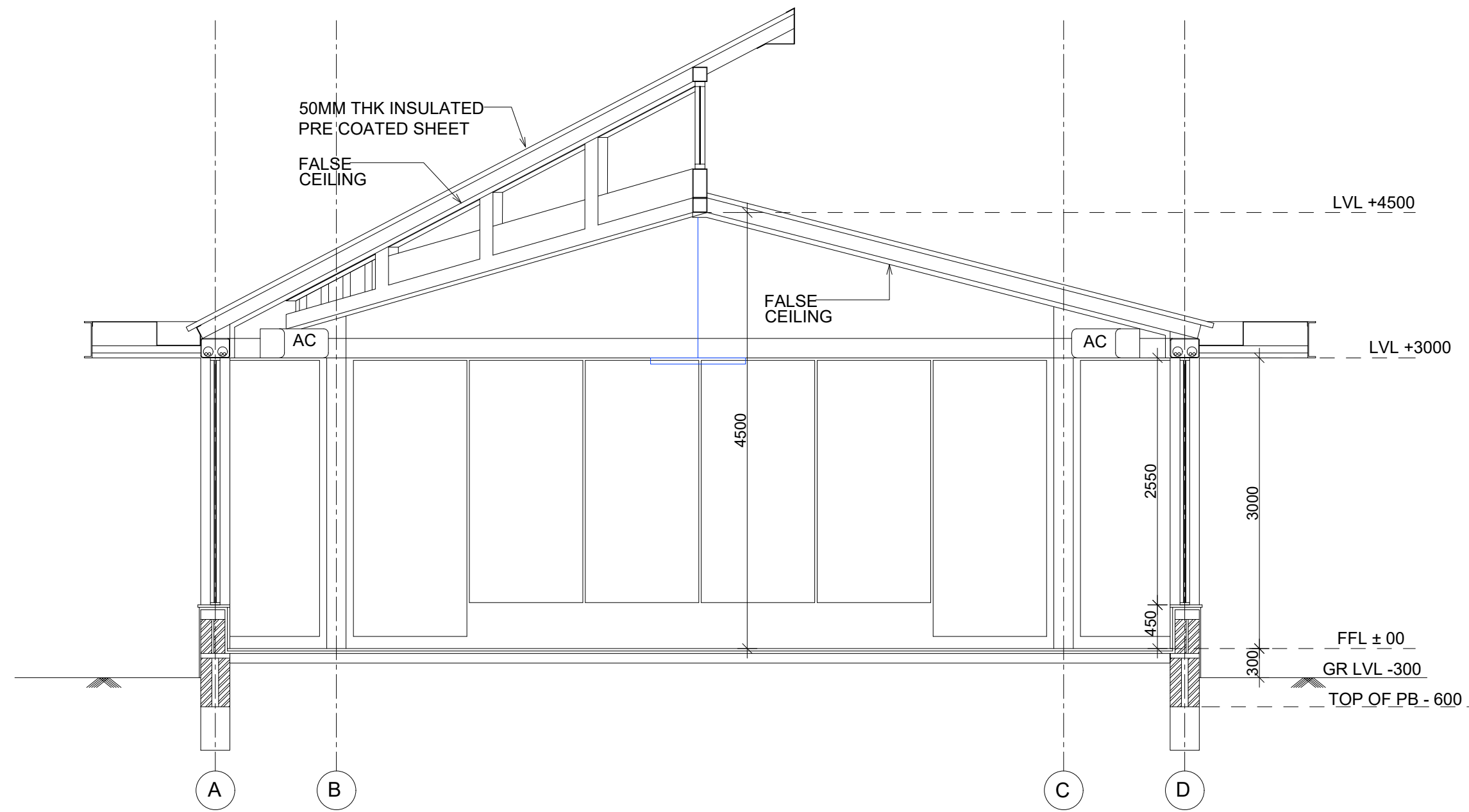
SECTION - AA
