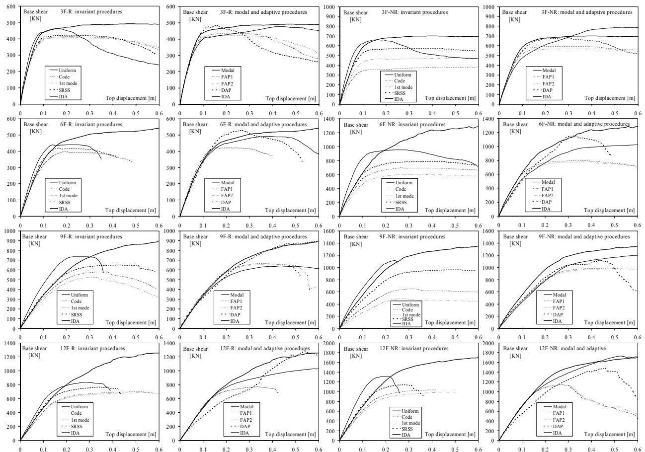
Figure 2 Base shear-top displacement curves
