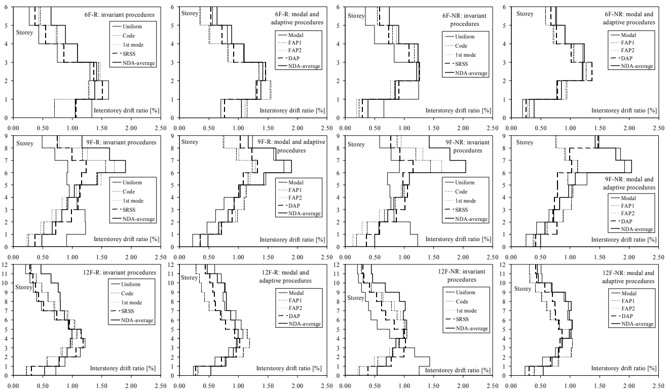
Figure 3 Inter-storey drift profiles
