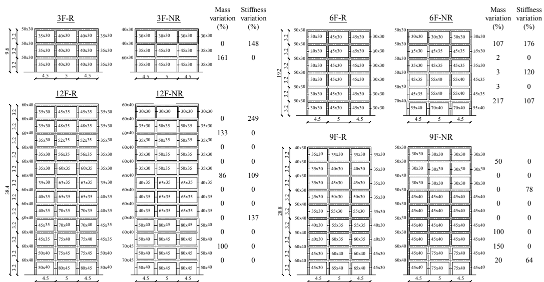
Figure 1 Structures under study (length and height in m, cross sections in cm)
