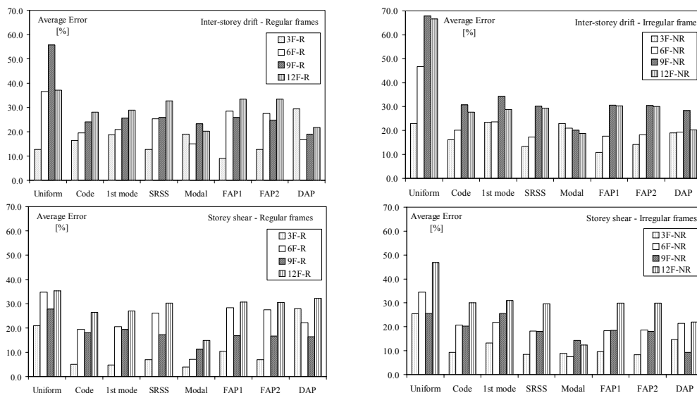
Figure 5 Average error in the prediction of inter-storey drift and storey shear
