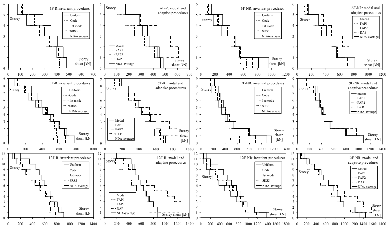
Figure 4 Storey shear profiles
