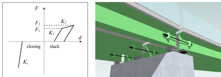
Figure 4 Analytical model of the cable restrainer
