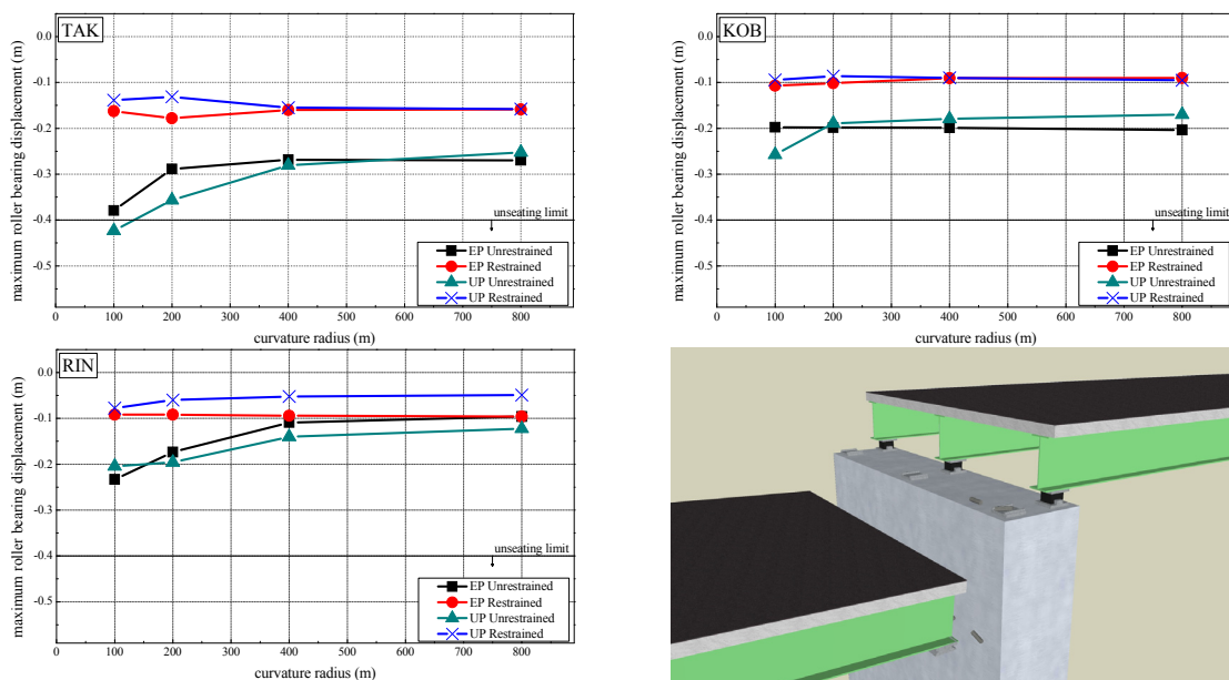
Figure 5 Curvature effect on deck unseating damage
