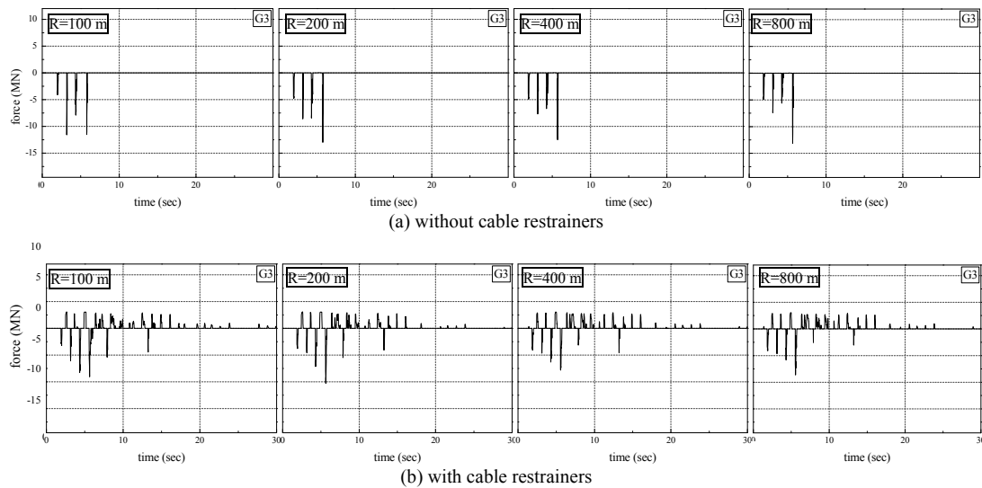
Figure 7 Impact forces at the expansion joint from TAK record in UP
