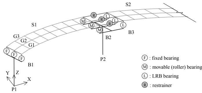
Figure 2 Detail of curved viaduct finite element model
