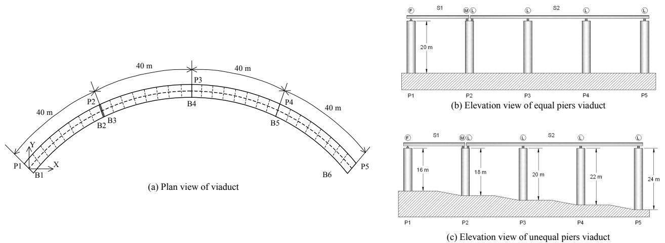
Figure 1 Model of curved highway viaduct
