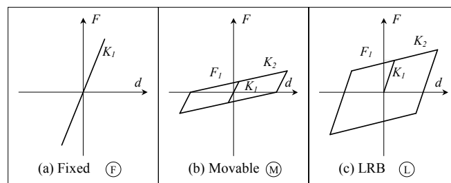
Figure 3 Analytical models of bearing supports
