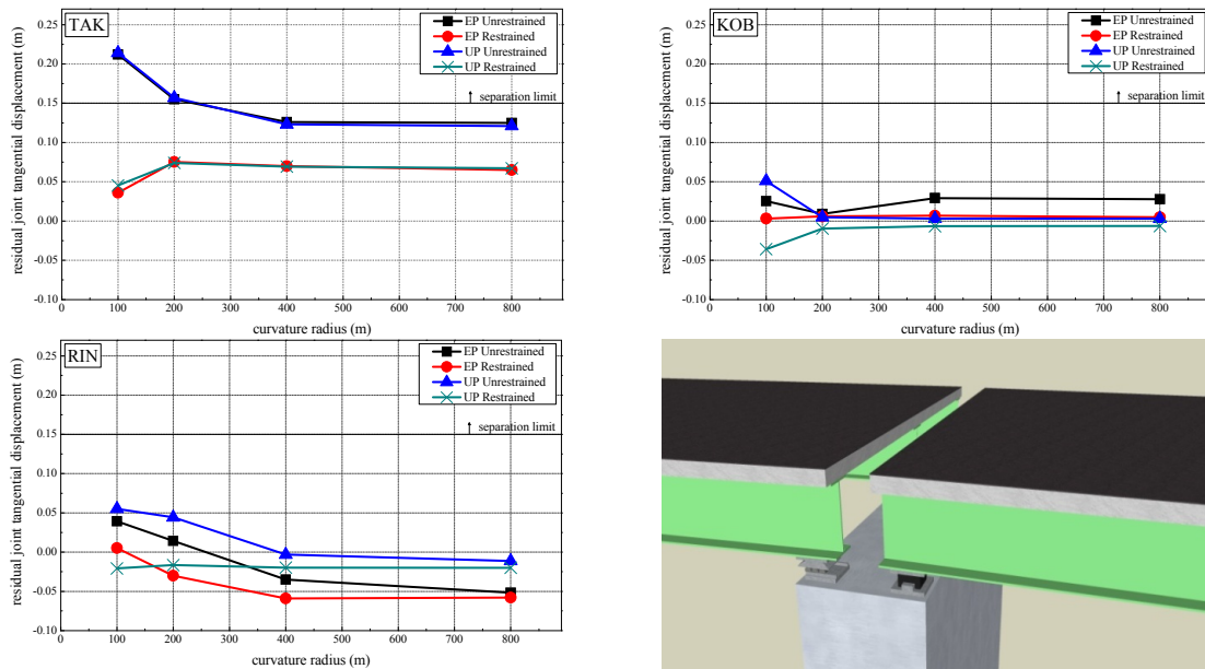
Figure 6 Effect of curvature radius on tangential joint residual damage
