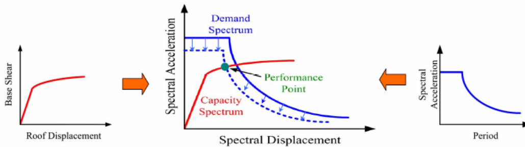
Fig2. Process of determining performance point
