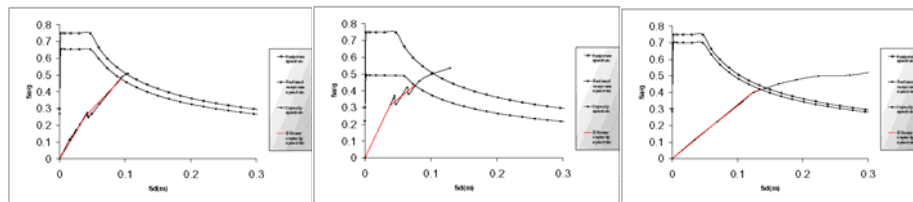
Figure No.8- performance point of frame 13 (Right hand). Frame 8 (middle). Frame 3 (left hand).
