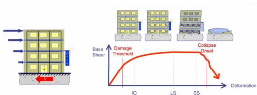
Fig1. Performance Level of Structure
