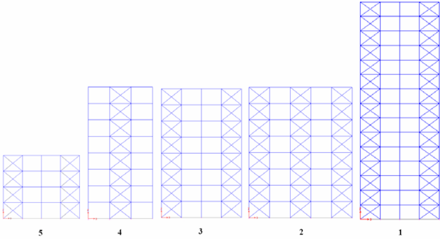
Fig.5-frames retrofitted by X-shaped brace.
