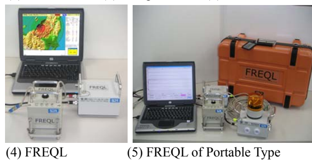
Fig.2 UrEDAS, Compact UrEDAS, FREQL and AcCo
