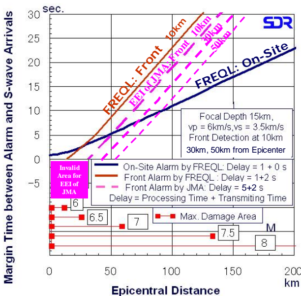
Fig.9 Margin time by EEW
