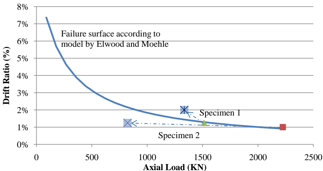
Figure 7. Relationship between drift ratio at axial failure and axial load for multiple failure events.
