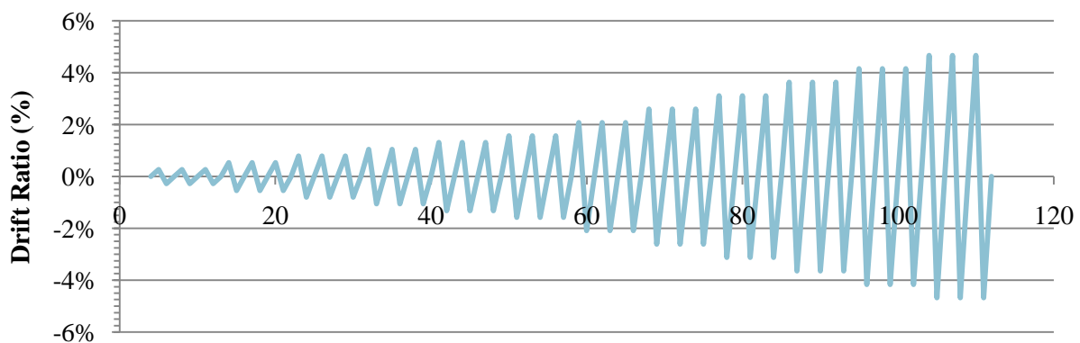
Figure 2 Lateral displacement protocol
