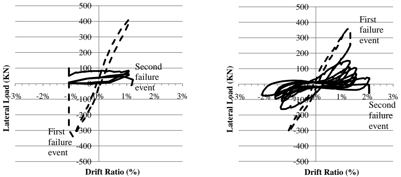
Figure 6. Load-deformation response for specimens 1 and 2 at drift demands beyond axial failure
