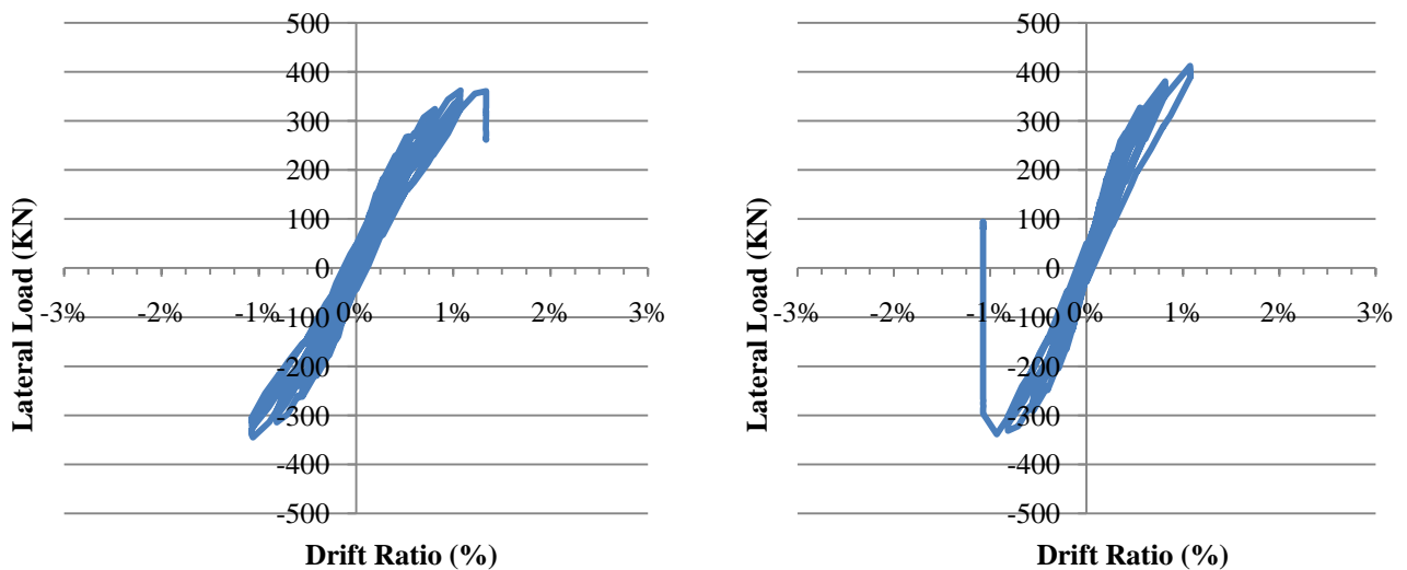
Figure 4. Load-Deflection relationship for Specimens 1 and 2
