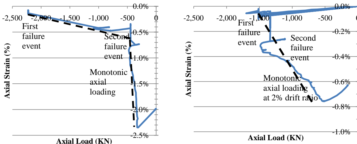
Figure 6. Axial strain vs. axial load for specimens 1 and 2
