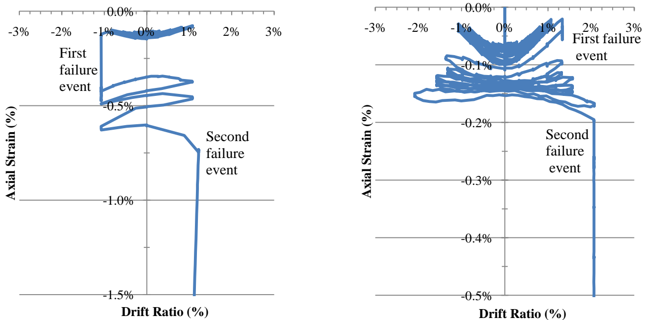
Figure 5. Axial strain vs. drift ratio for specimens 1 and 2.
