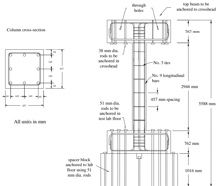
Figure 1 Specimen dimensions
