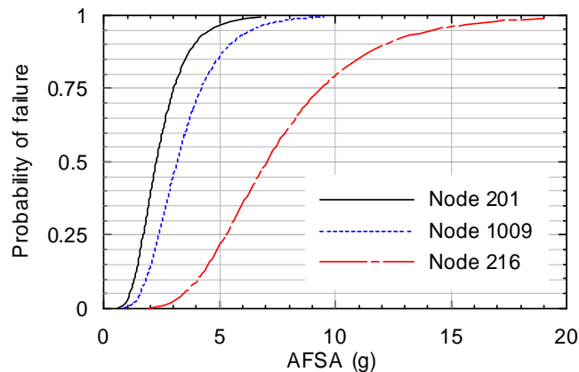
Figure 7. Mean fragility curves for the secondary systems at Nodes 201, 1009 and 216
