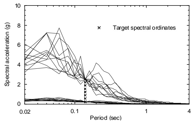
b. Response spectra of the ground motions in Bins TC1 and TC8
