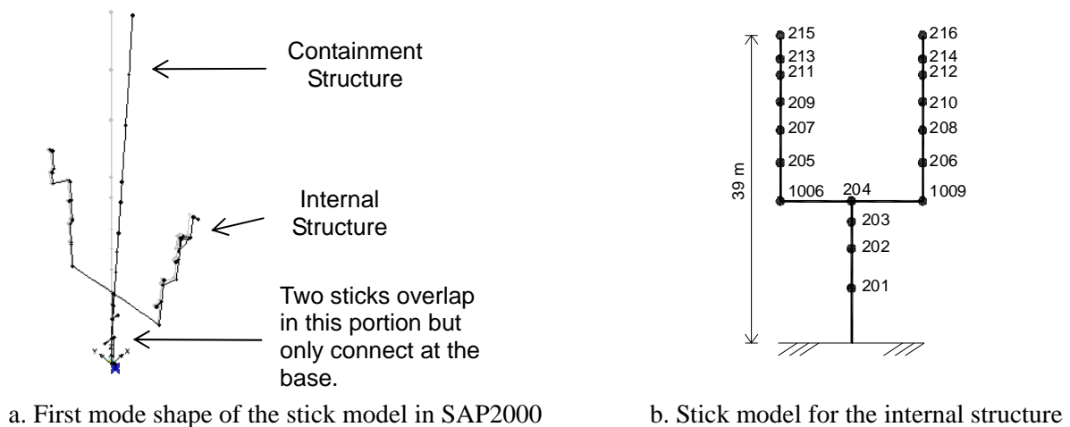
Figure 2. Stick model for the sample NPP reactor building
