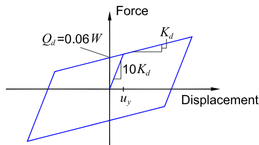
Figure 3. Assumed properties of the LR bearings
