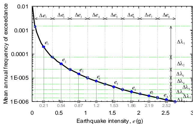
a. Computation of target spectral ordinates
