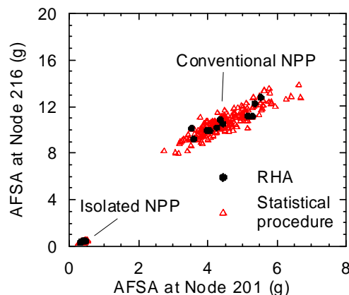
Figure 8. AFSA at Nodes 201 and 216 for 1) the conventional NPP to the Bin TC8 ground motions and 2) the isolated NPP to the Bin TI8 ground motions in the X direction
