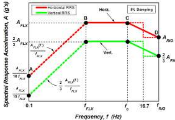
Figure 1 AC156 Required Response Spectrum Normalized for Nonstructural Components
