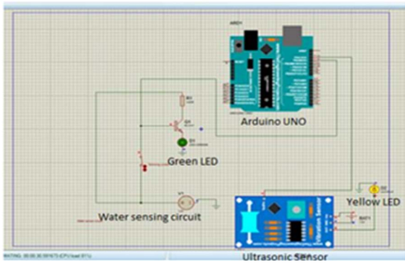
Fig. 5. Transmitter circuit simulation
