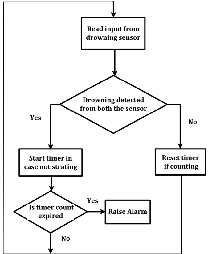
Fig. 4 Flow chart of Alarm trigger
