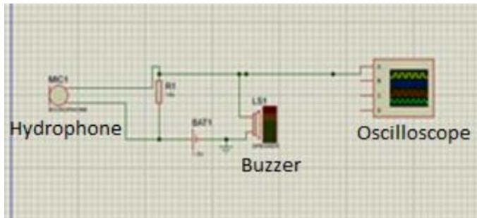
Fig. 6. Receiver circuit simulation
